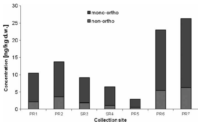
Figure 2 | Changes in concentrations of non-ortho and mono-ortho PCB congeners in sediment samples along the Pilica River (PR) and the Sulejow Reservoir (SR).
