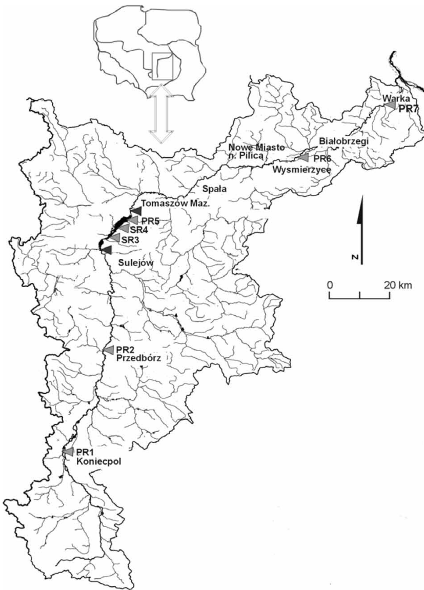
Figure 1 | Location of sediment sampling points (grey arrows: PR1, PR2, SR3, SR4, PR5, PR6 and PR7) and water samples (black arrows: below and above the reservoir) on the Pilica River and the Sulejow Reservoir.
