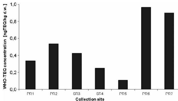
Figure 3 | Changes in WHO-TEQ concentration of dl-PCBs in sediment samples along the Pilica River (PR) and the Sulejow Reservoir (SR).
