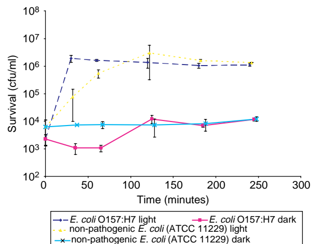
Figure 2 | Comparison of repair potential between E. coli O157:H7 and non-pathogenic E. coli (ATCC 11229) following LP UV irradiation at 8 mJ/cm 2 . Averages with standard deviations are shown.
