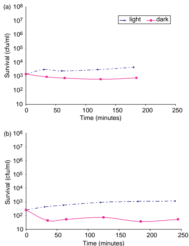
Figure 4 | Repair potential of E. coli O157:H7 following LP UV irradiation at (a) 20 and (b) 40 mJ/cm 2 . Representative experiments are shown.
