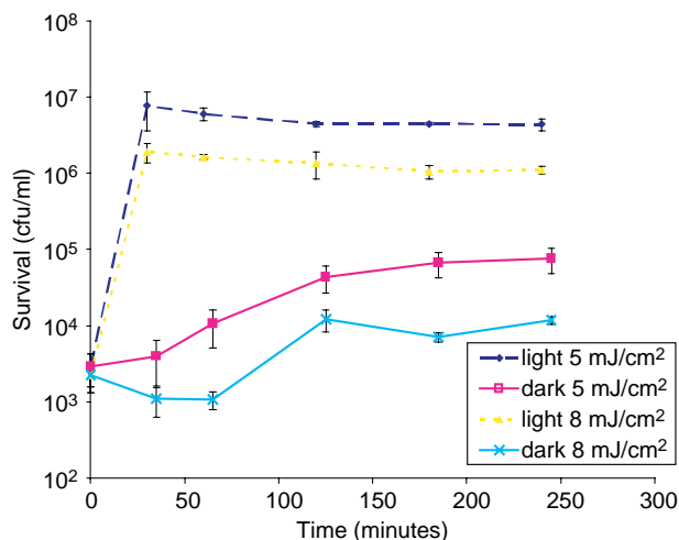
Figure 1 | Repair of E. coli O157:H7 following LP UV irradiation at low doses of 5 and 8 mJ/cm 2 . Averages with standard deviations at 5 mJ/cm 2 are based on three separate experiments and at 8 mJ/cm 2 are based on five separate experiments.
