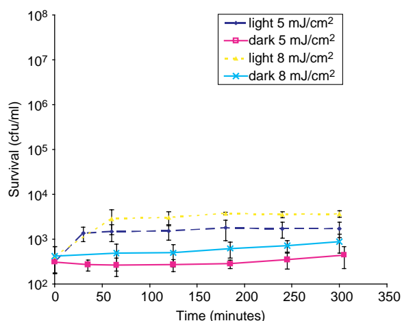
Figure 3 | Repair potential of E. coli O157:H7 following MP UV irradiation at weighted doses of 5 and 8 mJ/cm 2 . Averages with standard deviations at 5 mJ/cm 2 are based on four separate experiments and at 8 mJ/cm 2 are based on three separate experiments.
