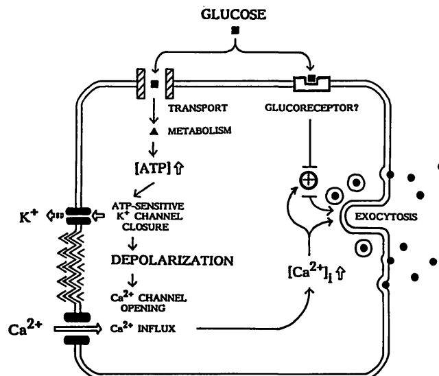
FIG. 7. Schema for dual functional role of membrane depolarization/ \text{Ca}^{2+} influx. Depolarization is caused by \text{K}^+_{\text{ATP}} channel closure due to increase of ATP. Opening of the voltage-dependent \text{Ca}^{2+} channel ensue and cytosolic free \text{Ca}^{2+} ( [\text{Ca}^{2+}]_i ) rises as a result of \text{Ca}^{2+} influx. It stimulates exocytosis through \text{Ca}^{2+} -dependent mechanisms on one hand and induces the coupling of another glucose-responsive effector and the process of exocytosis on the other.
