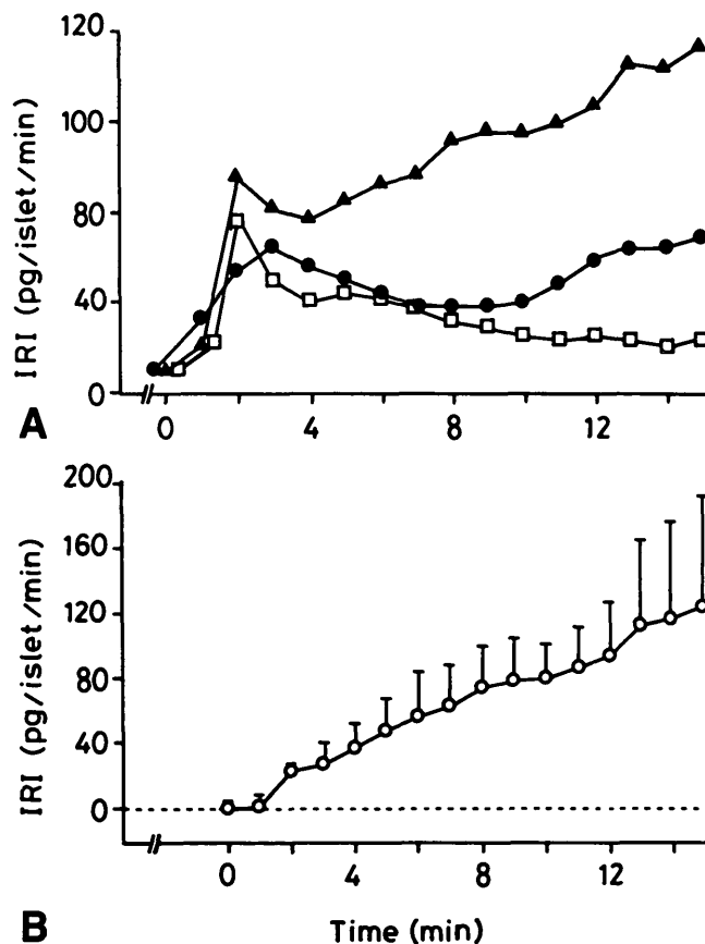
FIG. 2. A : immunoreactive insulin (IRI) secretion in response to 16.7 mM glucose [G 16.7 ] (●), 50 mM K + [K + 50 ] (□), and [K + 50 + G 16.7 ] (▲). B : subtraction of the response to [K + 50 ] from that to [K + 50 + G 16.7 ] yields gradually increasing IRI secretion. Data shown were obtained with the same batch of islets (for details of experimental procedure, see METHODS). For clarity, mean values of 3–5 columns are shown, and SD (86% of the mean at most) has been omitted in all perfusion results except in B . Stimulation is started at time 0 min after stabilization of basal secretion in all perfusion experiments. Conversion factor of IRI to SI units is 0.1739 (pg/islet/min → nmol/islet/min).
