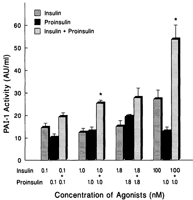
FIG. 3. PAI-1 activity in porcine aortic endothelial cells in conditioned media 24 h after adding of insulin alone, proinsulin alone, and the combination of insulin and proinsulin. PAI-1 activity in media from control cells averaged 2.0 \pm 0.6 AU/ml. Values are means \pm SE. * P < 0.02 compared with insulin alone and with proinsulin alone.
