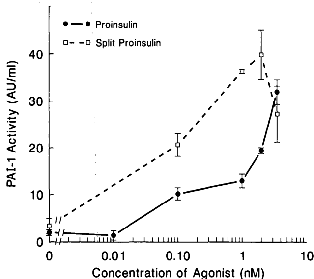
FIG. 1. PAI-1 activity in porcine aortic endothelial cells in conditioned media 24 h after adding proinsulin or split proinsulin (means \pm SE). All increases over control (0 nM) were significant ( P < 0.05 ) except for those seen with 0.01 nM proinsulin.
