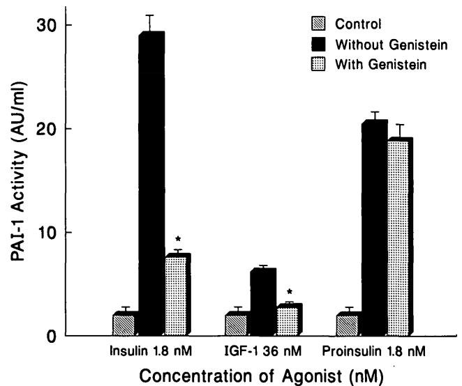
FIG. 5. PAI-1 activity in porcine aortic endothelial cells in conditioned media 24 h after adding insulin, IGF-I, and proinsulin with and without exposure of the cells to 40 \mu\text{g/ml} of genistein for 30 min at time 0. Values are means \pm SE. * P < 0.01 compared with results in cells that were not exposed to genistein.
