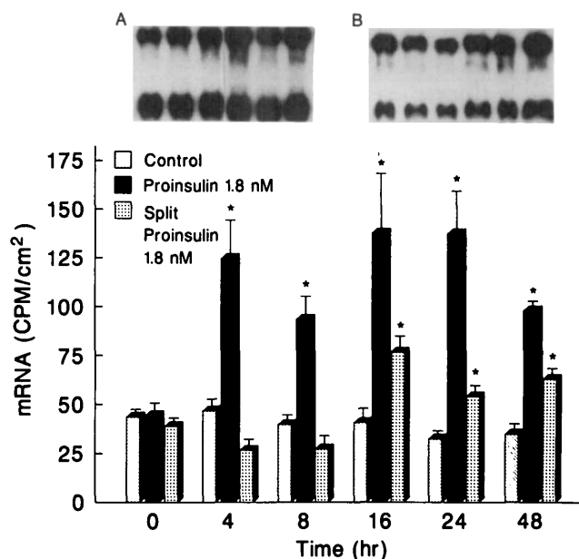
FIG. 2. PAI-1 mRNA expression in porcine aortic endothelial control cells and cells exposed to 1.8 nM proinsulin or 1.8 nM split proinsulin. The inset shows a representative autoradiogram (A, proinsulin; B, split proinsulin). The top 2 bands are 3.2 and 2.2 kb PAI-1 mRNA that were summed for quantification. The third band is glyceraldehyde-3-phosphate dehydrogenase mRNA. Values are means \pm SE. * P < 0.02 compared with control mRNA.
