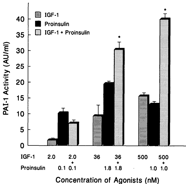
FIG. 4. PAI-1 activity in porcine aortic endothelial cells in conditioned media 24 h after adding IGF-I alone, proinsulin alone, and the combination of IGF-I and proinsulin. PAI-1 activity in media from control cells averaged 2.0 \pm 0.6 AU/ml. Values are means \pm SE. * P < 0.01 when compared with IGF-I alone and with proinsulin alone.
