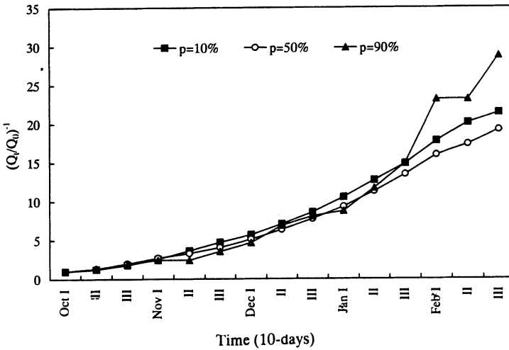
Fig. 2. Checking the Blue Nile recession patterns with b = 1 .
