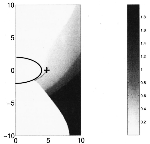
FIG. 2. Same as Fig. 1 but for the hyperbolicity persistence d_T^+(x_0) of the velocity gradient tensor expressed in strain basis.
