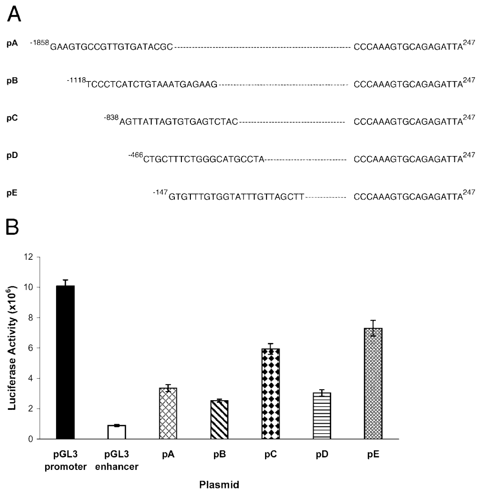
FIGURE 3. Effect of the human IL-19 promoter on luciferase activity. Potential transcription start site was designated as nucleotide 1. A, Five fragments (pA, pB, pC, pD, pE) containing different lengths of sequences upstream of exon 1 and 247 bp of exon 1 were ligated into the vector of the promoterless luciferase gene (pGL3 enhancer). pA contains 2105 bp (from -1858 to 247). pB contains 1365 bp (from -1118 to 247). pC contains 1085 bp (from -838 to 247). pD contains 713 bp (from -466 to 247). pE contains 394 bp (from -147 to 247). B, These five fusion genes were transfected into the MDCK cells, along with the negative control promoterless vector (pGL3 enhancer) and the positive control vector (pGL3 promoter). The luciferase activity data presented here are averages of triplicate samples.
