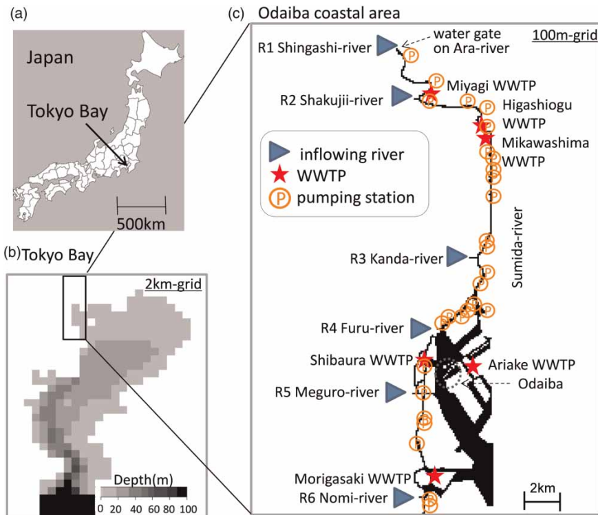
Figure 1 | Schematic of the study area: (a) Japan area, (b) Tokyo Bay area and (c) Odaiba coastal area including location of rivers, WWTPs and pumping stations.
