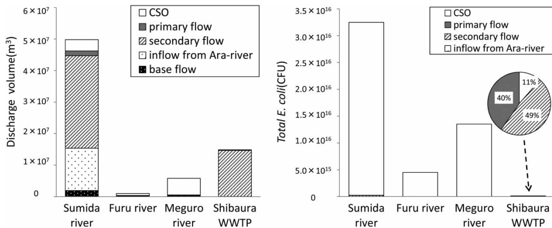
Figure 4 | Total discharge volume (left) and E. coli (right) from Sumida River, Furu River, Meguro River and Shibaura WWTP during 20 days (8–27 November).
