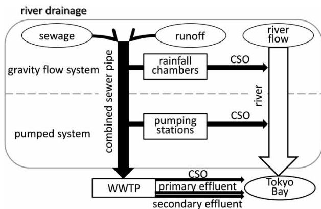
Figure 2 | Conceptual diagram of CSO discharge in combined sewer system.
