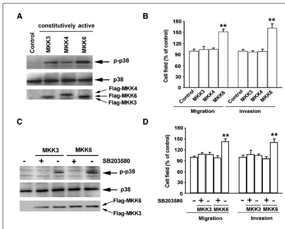
Figure 5. Constitutively active MKK6 renders siPKC \alpha -SK cell migratory and invasive phenotypes. A , effects of transfection with MAPKKs. siPKC \alpha -SK was transfected with constitutively active MKK3, MKK4, and MKK6 vector for 48 h. The cells were lysed, and Western blotting was done to detect phosphorylated p38 MAPK, p38 MAPK, and flag-tagged MAPKKs. B , migratory and invasive potentials in cells transfected with MAPKKs. Migration and invasion assays were done on the siPKC \alpha -SK cells transfected with constitutively active MKK3, MKK4, and MKK6 vector and vector. **, P < 0.01 versus control. C , effects of p38 MAPK inhibitor SB203580 on cells transfected with MAPKKs. siPKC \alpha -SK was transfected with constitutively active MKK3 or MKK6 vector for 48 h. SB203580 (50 \mu mol/L) was then added to the cells for 24 h and subsequently lysed for Western blotting to detect phosphorylated p38 MAPK, p38 MAPK, and flag-tagged MAPKKs. D , migratory and invasive potentials in cells transfected with MAPKKs and treated with SB203580. Migration and invasion assays were done on the siPKC \alpha -SK transfected with constitutively active MKK3, MKK6, or vector, and SB203580 (50 \mu mol/L) was then incubated with the cells for 24 h. **, P < 0.01 versus control.
