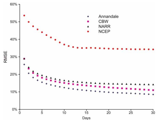
Figure 5 | Mean total RMS error (percent) versus number of days for estimation of Q_{\text{siD}} during March and April.
