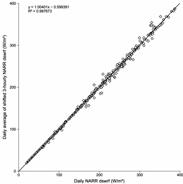
Figure 2 | Daily downward shortwave radiation flux (dsrwr) calculated from three-hour data shifted backwards six hours versus daily values. Data for Edmonton, AB (2000).
