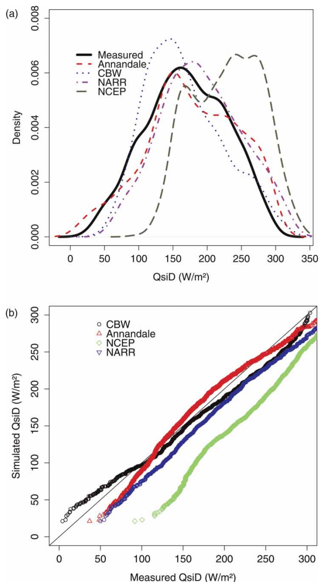
Figure 6 | Plots describing frequency distributions of Edmonton measured and simulated Q_{siD} . (a) Kernel density plots of Edmonton measured, Annandale, CBW, NARR, and NCEP Q_{siD} . (b) Quantile–quantile plots of Edmonton spring Annandale, CBW, NARR, and NCEP Q_{siD} , against measured quantiles. The line is 1:1.
