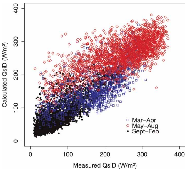
Figure 4 | Annandale calculated Q_{\text{siD}} vs measured Q_{\text{siD}} (W/m 2 ) for Winnipeg during snowmelt (Mar-Apr), growing (May-Aug) and dormant (Sept-Feb) seasons.
