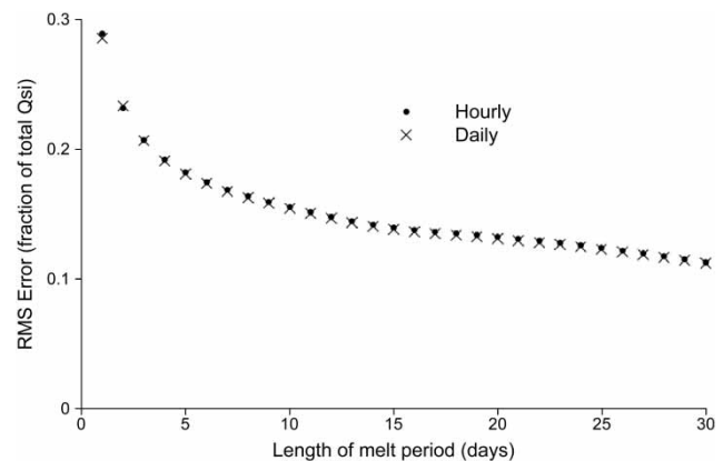
Figure 10 | RMS Error as a fraction of total Q_{si} , for cumulative hourly and daily Winnipeg Annandale estimates.
