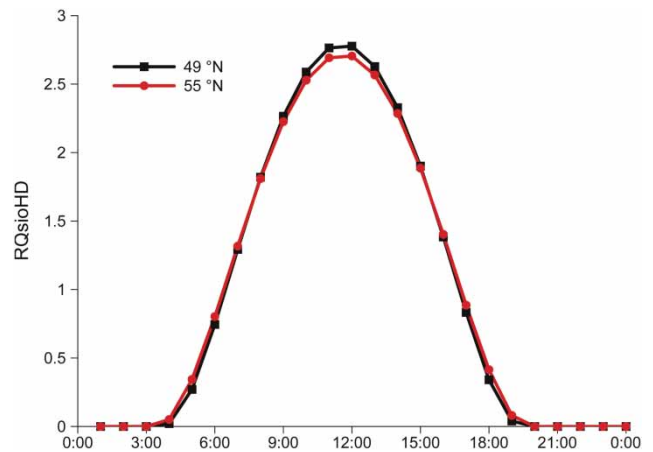
Figure 8 | Hourly values of R_{Q_{\text{siOHHD}}} (the ratio of Q_{\text{siH}} to Q_{\text{siOD}} ), computed for latitudes 49° and 55°N, for day number 172 (June 21, for non-leap year).
