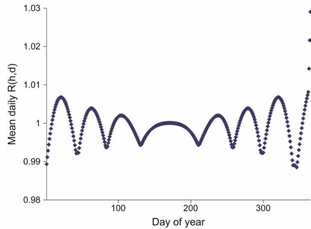
Figure 9 | Mean daily value of R(h,d) versus day of year.
