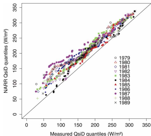
Figure 7 | Quantiles of simulated versus measured Q_{siD} for Swift Current, by year.
