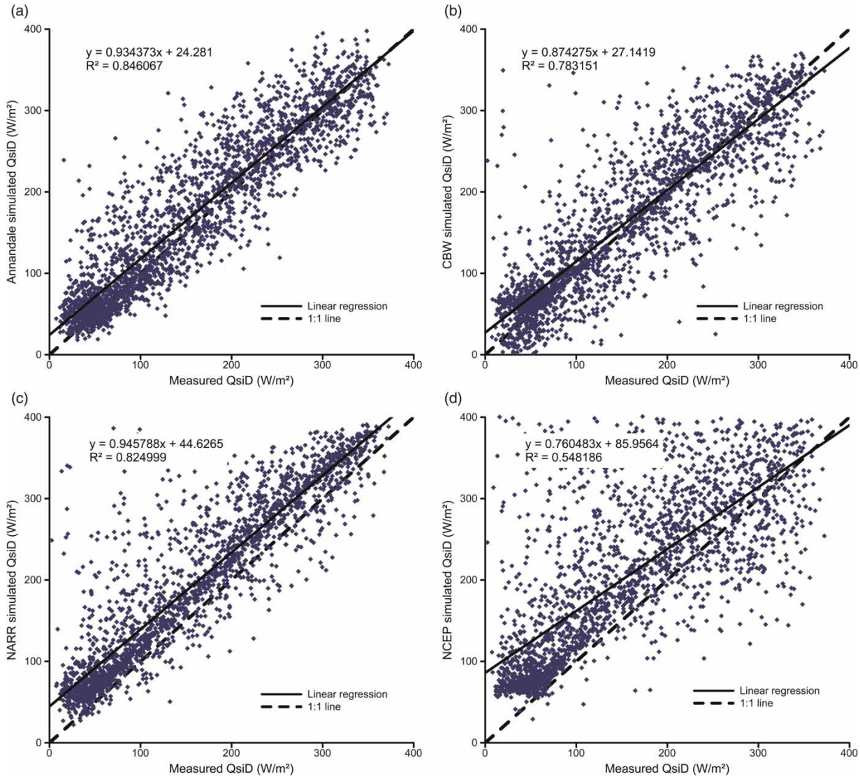
Figure 3 | Simulated Q_{sID} by (a) Annandale, (b) CBW, (c) NARR, and (d) NCEP versus measured for Lethbridge.
