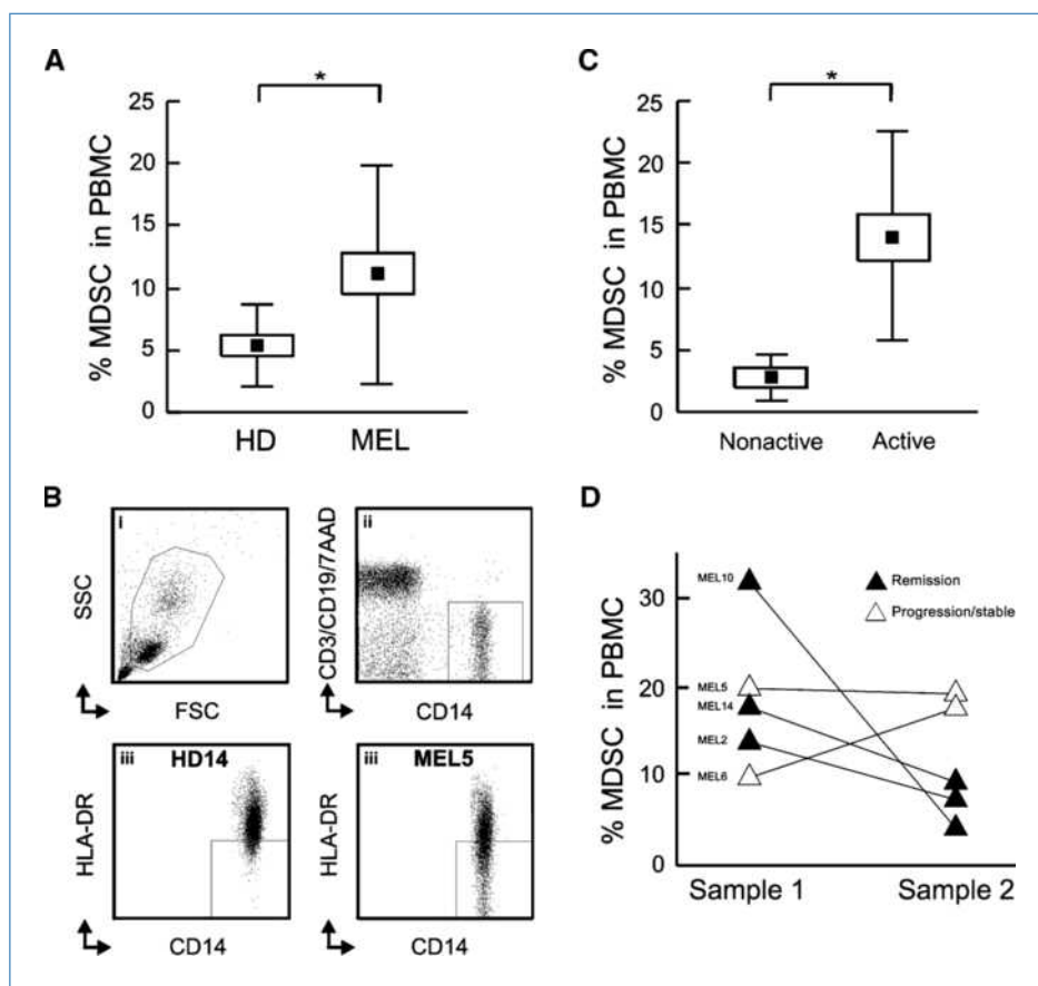
Figure 1. MDSC are increased in PBMCs of patients with melanoma. Flow cytometry shows that CD14 + HLA-DR -low cell frequencies (A) are increased in MM (MEL; n = 31 ) versus healthy donor (HD; n = 15 ) PBMCs, with (B) decreased HLA-DR expression on MM (bottom right) versus healthy donor (bottom left) CD14 + cells; top, gating strategy from (i) PBMCs (top left) to (ii) CD14 + (CD3 + CD19 - 7AAD - ) cells (top right). C, higher MDSC frequencies are observed in patients with active ( n = 25 ) versus nonactive ( n = 7 ) disease. D, correlation of MDSC with disease course in patients with tumor reduction or progression. Points, mean; bars, SEM; *, P < 0.05 .
