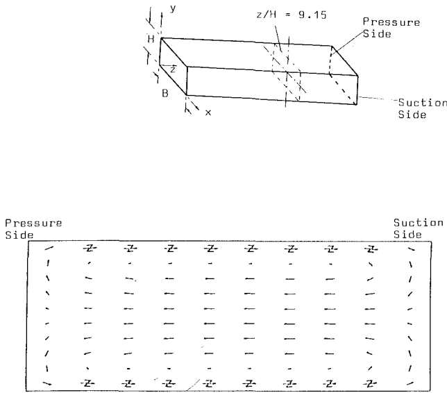
Fig. 16 Predicted secondary velocity field for \Omega B/\bar{\omega} = .22 at z/H = 9.15
