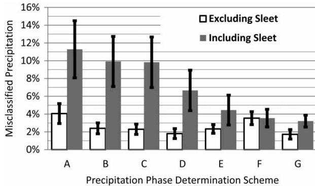
Figure 5 | Misclassified precipitation from -1 to 5 °C with error bars representing the standard deviation from the 19 meteorological stations.
