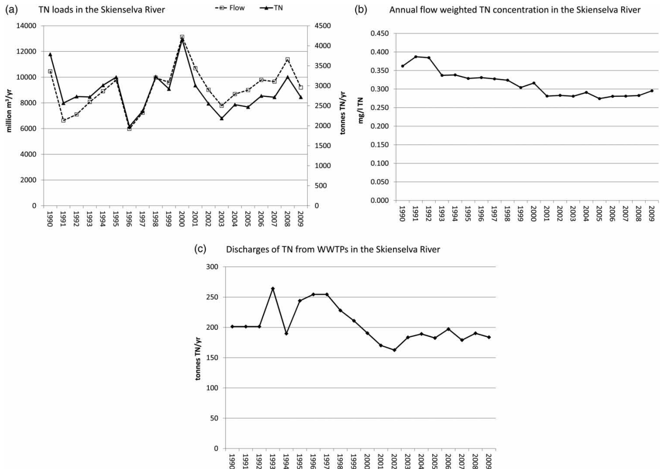
Figure 2 | Data on the Skienselva catchment showing riverine TN loads (tonnes) and water flow (mill \text{m}^3/\text{yr} ) (a); annual flow-weighted TN concentrations ( \text{mg}/\text{L} ) (b); and TN effluents (tonnes) from WWTPs (c).
