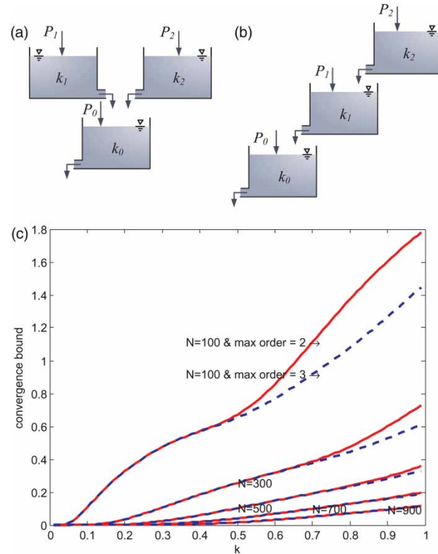
Figure 4 | (a) and (b) show the two configurations with R = 3 , (a) has a maximum order of 2 while (b) has a maximum order of 3. (c) shows how the convergence bound (the RHS of the probability inequality in Theorem 2) for these two models performs when the recession coefficient is spatially constant (i.e., k_1 = k_2 = k_3 = k , k is varied over a range [0.01, 0.99] and N in (\delta/\eta)^2(N/2R^2) is varied {100, 300, 500, 700, 900} ( \delta/\eta = 0.1 , R = 3 ). P_i denotes effective precipitation (input going into the store i ). In (c), 'Max order = 2' refers to the model in (a) with maximum order of reservoir = 2 and 'Max order = 3' refers to the model in (b).
