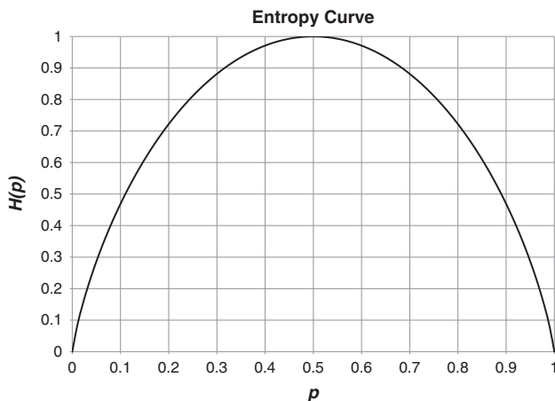
Figure 5 | Entropy curve for the realized probability p of a random variable X .
