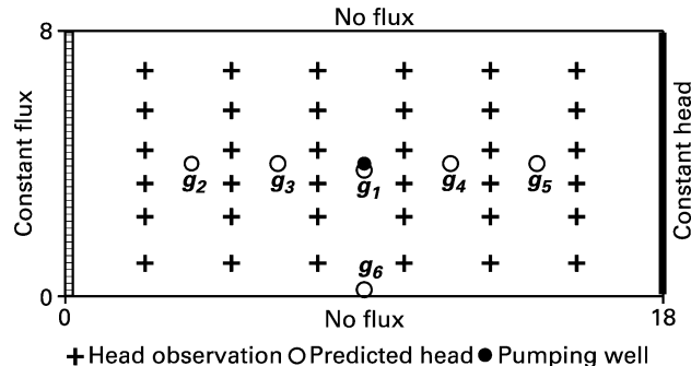
Figure 1 Domain, boundary conditions, observations and predictions for flow models
