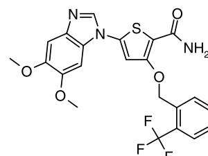
Structure of Compound 1
