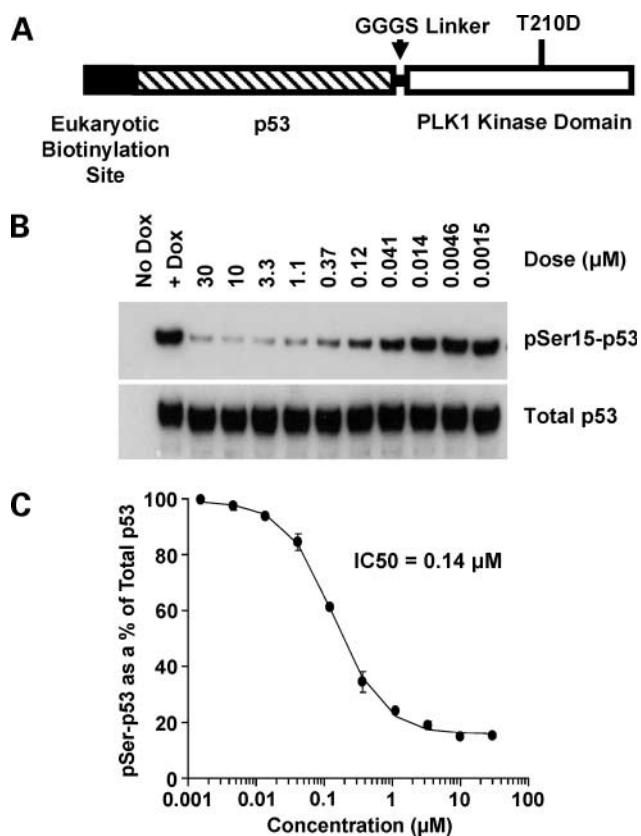
Figure 1. Mechanistic cellular assay for PLK1. A , schematic diagram of the tet -inducible chimeric p53-PLK1 protein. The chimeric protein has a eukaryotic biotinylation site at the NH 2 terminus, which allows binding to streptavidin, and a flexible GGGG linker to facilitate intramolecular phosphorylation. The p53 comprises the entire protein, and the PLK1 sequence encompasses amino acids 3 to 345, which include the kinase domain but not the polo boxes. B , Western immunoblots of HeLa cells treated with compound 1 following induction of the p53-PLK1 fusion. Top , phospho-p53 (Ser 15 ); bottom , total p53. C , compound 1 inhibition curve from an ELISA developed using the tet -inducible p53-PLK1 fusion protein expressed in HeLa cells (IC 50 , 0.14 μmol/L).
