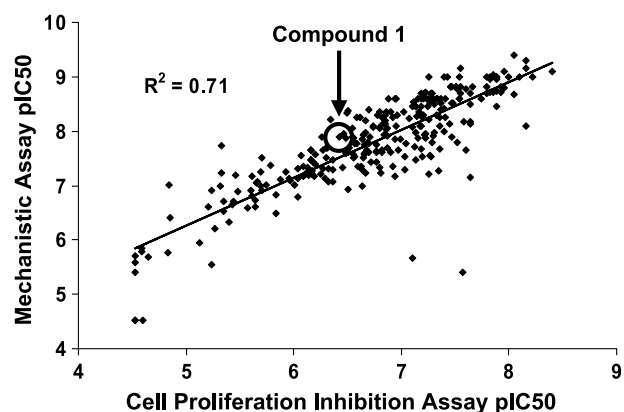
Figure 2. Graph showing the correlation between the pIC 50 s of the methylene blue cell proliferation assay and the mechanistic assay of compounds screened in both assays. The data for the methylene blue assay are from H460 cells and the mechanistic assay data are from HeLa cells expressing the tet -inducible chimeric p53-PLK1 protein. Compound 1 is indicated on the plot. The pIC 50 is calculated as -\log_{10}(\text{IC}_{50}) .
