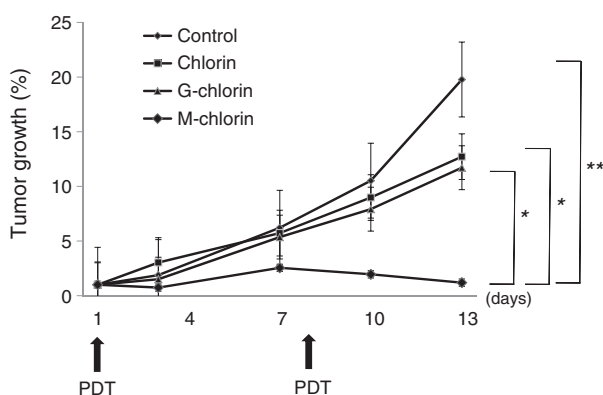
Figure 5. Antitumor effects of PDT in mouse allograft model. Mice were irradiated with 13.9 \text{ J/cm}^2 of LED light at 660 nm 24 hours after injection of the photosensitizer. PDT was performed on day 1 and day 8, and tumor volumes were monitored for 13 days in total. Data are means \pm SE ( n = 4 for control, n = 5 for chlorin, G-chlorin, and M-chlorin). *, P < 0.05 ; **, P < 0.01 .
