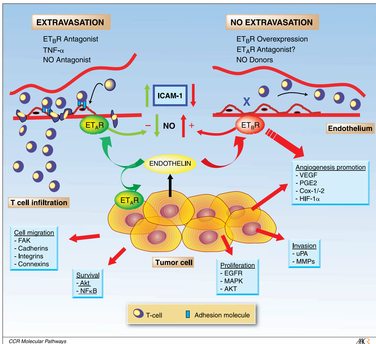
Fig. 1. Control of T-cell homing to tumors by endothelin 1 expressed by tumor cells. Opposite paracrine effects are exerted by endothelin on tumor endothelium through ET_A R and ET_B R. The balance between ET_A R and ET_B R determines the fate of antitumor T-cell response. Overexpression of ET_B R in tumor endothelium results in increased angiogenesis but also suppression of ICAM-1 expression on endothelial cells, and inhibition of T-cell transendothelial migration and homing. This effect is largely mediated by NO. NO donors and possibly ET_A R inhibitors exert similar effects. ET_B R blockade results in increased expression of endothelial ICAM-1 and increased binding and transendothelial migration of T cells to the tumor. NO antagonists and TNF- \alpha exert similar effects. Additional tumor-promoting autocrine effects of endothelin are established by binding to ET_A R on tumor cells, resulting in enhanced tumor cell survival, proliferation, migration, and invasion. Each of these effects entail multiple signaling pathways.
