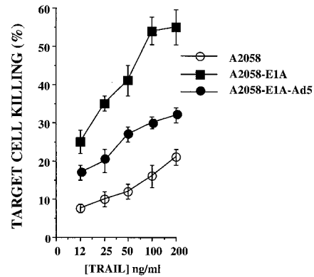
FIGURE 3. Ad5-infection inhibits TRAIL-dependent killing of E1A-transfected cells. Parental and E1A-transfected A2058 cells were mock or Ad5-infected for 16 h and their sensitivity to TRAIL-induced killing was determined in a 16-h cytotoxicity assay. TRAIL-induced lysis of A2058 (○), Ad5-infected A2058-E1A (●), or uninfected A2058-E1A cells (■).
