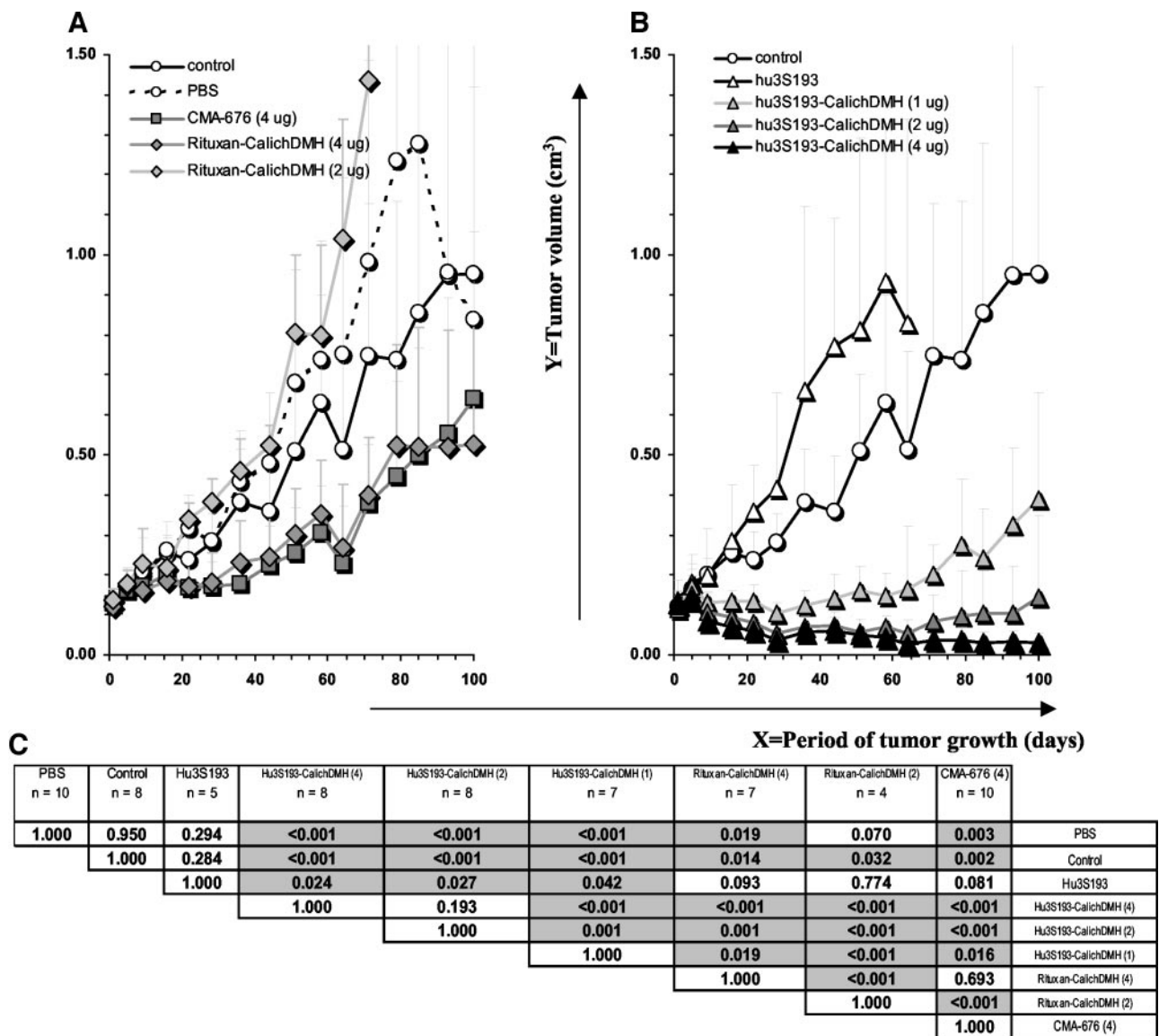
Fig. 5 Inhibition of N87 tumor growth by hu3S193- N -acetyl \gamma calicheamicin dimethyl hydrazide ( CalichDMH ). Mice bearing N87 [Lewis (Le) + , CD33 - , and CD20 - ] xenografts of 100 mm 3 were treated with control conjugates (CMA, rituxan- CalichDMH ), PBS, hu3S193, or hu3S193- CalichDMH . Mice in each group received three doses i.p. The amount of each dose in calicheamicin equivalents is specified in the legend. Conjugates and controls were injected at days 1, 5, and 9. A shows the efficacy of control conjugates. B illustrates the effects of hu3S193 and of its CalichDMH conjugate. Bars , SD of the average tumor volume at each time point. Differences in tumor size among the treated groups of tumor bearing mice have been probed by a 2-tailed Student's t test. The P -values at day 28 are shown in C . n = number of mice per group.
