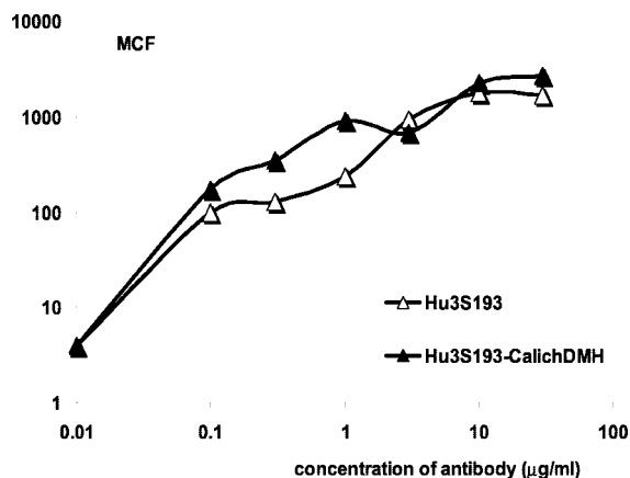
Fig. 3 Comparison of the binding of hu3S193 and hu3S193- N -acetyl \gamma calicheamicin dimethyl hydrazide ( CalichDMH ) by fluorescence-activated cell sorter analysis. N87 cells were incubated with various concentrations ( X -axis) of hu3S193 or hu3S193- CalichDMH . The amount of bound conjugate or antibody was expressed as mean channel fluorescence ( MCF , Y -axis). The MCF represents the average fluorescent intensity of a cell population after binding of the primary antibody and the consecutive staining with a fluorescent-labeled secondary antibody.
