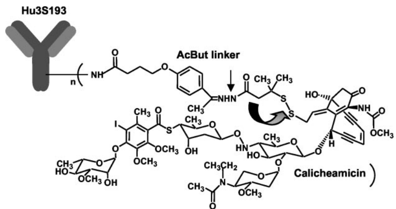
Fig. 1 Chemical structure of hu3S193- N -acetyl \gamma calicheamicin dimethyl hydrazide (Calich-DMH). Calicheamicin was bound to lysine residues of hu3S193 by an acid-hydrolyzable linker ( AcBut ). Release of CalichDMH from the antibody occurs at the hydrazone bond (straight arrow). Activation of the enediyne “warhead” is induced by reduction of the -S-S-bond (curved arrow). Conjugates with an average of 2 or 3 molecules of CalichDMH per antibody were used for the presented experiments.
