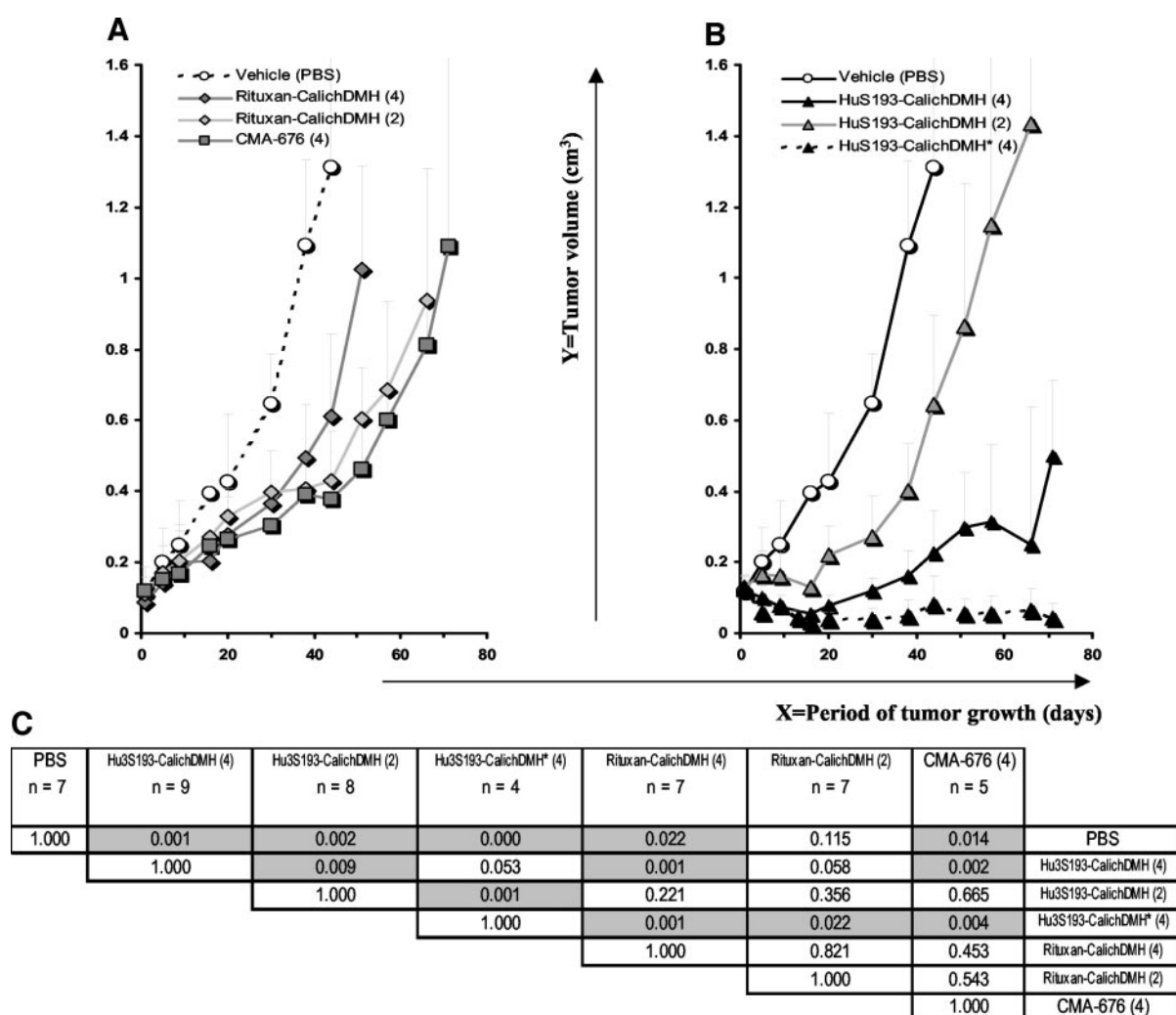
Fig. 8 Comparison of tumor growth inhibition by huS193-N-acetyl \gamma calicheamicin dimethyl hydrazide (CalichDMH) administered at 4 \mu g Q4Dx3 or Q4Dx4. Mice bearing LOVO xenografts of 100 mm 3 were treated with control conjugates: Rituxan-CalichDMH and CMA (A), PBS (A and B), or huS193-CalichDMH (B). Mice in each group received three or four doses i.p. The amount ( \mu g) of each dose in calicheamicin equivalents is specified in the legend. Conjugates and controls were injected at days 1, 5, and 9. The group designated huS193-CalichDMH*, received an additional dose at day 13. The number of mice per group (n) and P-values of a 2-tailed Student's t test are indicated in C.
