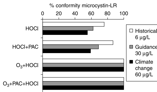
Figure 5 | Percentage of treatment trains able to lower microcystin-LR concentration under the acceptable limit of 1.5 \mu\text{g/L} considering the three source water occurrence scenarios.
