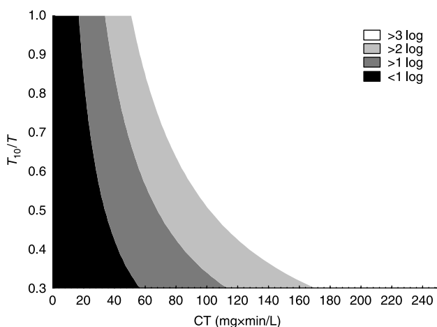
Figure 1 | Predicted microcystin-LR reduction (in log) by KMnO_4 for various CT and hydraulic efficiency factors ( T_{10}/T ) at 20°C (pH independent).
