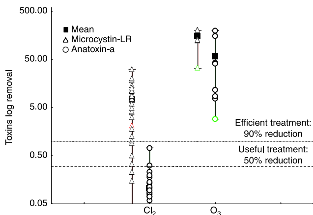
Figure 4 | Microcystin-LR and anatoxin-a log removals by chlorine (HOCL) and ozone in the sub-sample group.
