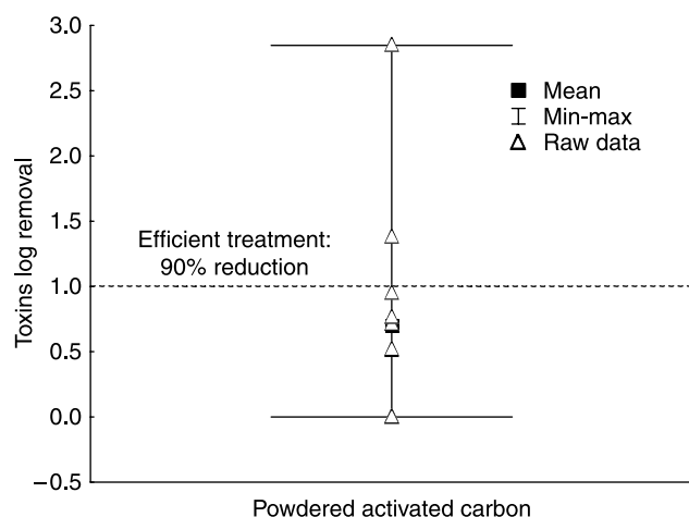
Figure 3 | Cyanotoxins log removal by powder activated carbon application in the sub-sample group.
