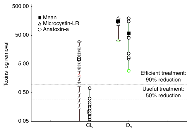
Figure 4 | Microcystin-LR and anatoxin-a log removals by chlorine (HOCL) and ozone in the sub-sample group.
