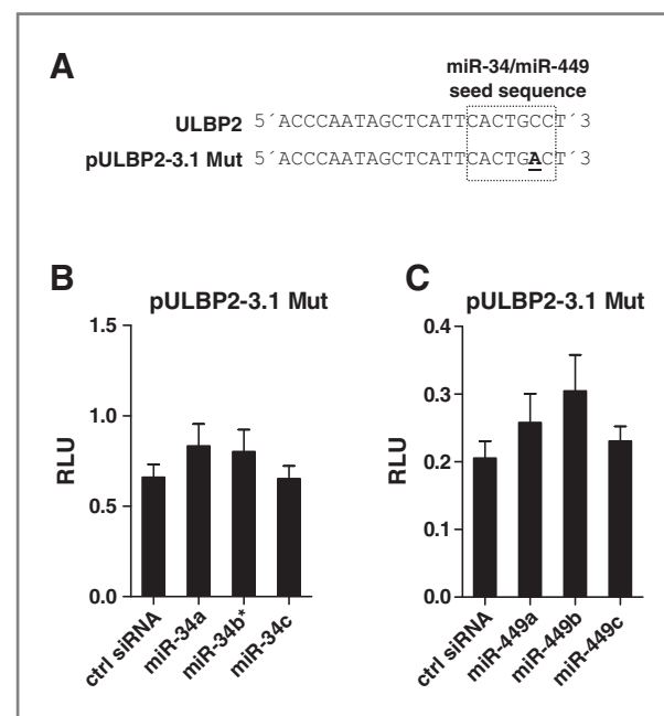
Figure 2. Specific mutation of the ULBP2 3'-UTR relieves from miR-34/miR-449-mediated repression. A , a point mutation was introduced into the ULBP2 3'-UTR of pULBP2-3.1 to destroy the predicted miR-34/miR-449-binding motif. The mutated plasmid was designated pULBP2-3.1 Mut. B and C , luciferase activity of pULBP2-3.1 Mut is not affected by transfection of miR-34 and miR-449 mimics. Data of normalized Renilla luciferase activity (RLU) represent means (+ SEM) of n = 3 experiments.
