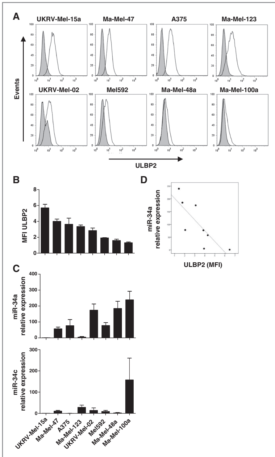
Figure 3. Expression of miR-34a and ULBP2 surface molecules inversely correlate. A and B , ULBP2 surface expression on different melanoma cell lines ( n = 8 ) was measured by flow cytometry. A , representative histograms of ULBP2 expression on melanoma cells. B , data are shown as mean MFI (+ SEM) of n = 3 experiments. C , cells were analyzed for miR-34a and miR-34c expression levels by qRT-PCR. miRNA expression was normalized to endogenous RNU6B. Expression levels, given as means (+ SEM) of n = 3 experiments, are indicated relative to the expression in UKRV-Mel-15a cells. D , statistical analysis revealed a significant negative correlation between expression levels of miR-34a and ULBP2 surface molecules (Spearman, P < 0.01 ).
