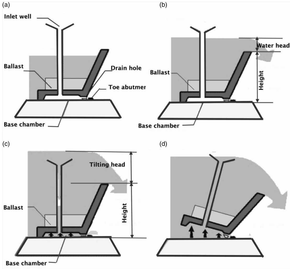
Figure 2 | Fusegate's cross-sections through a fusegate: (a) the water level is increasing, (b) fusegate acts as an ungated spillway, (c) the water head reaches to the predetermined elevation (design tipping head), and (d) the fusegate tips (Adapted from Hydroplus site www.hydroplus.com ).
