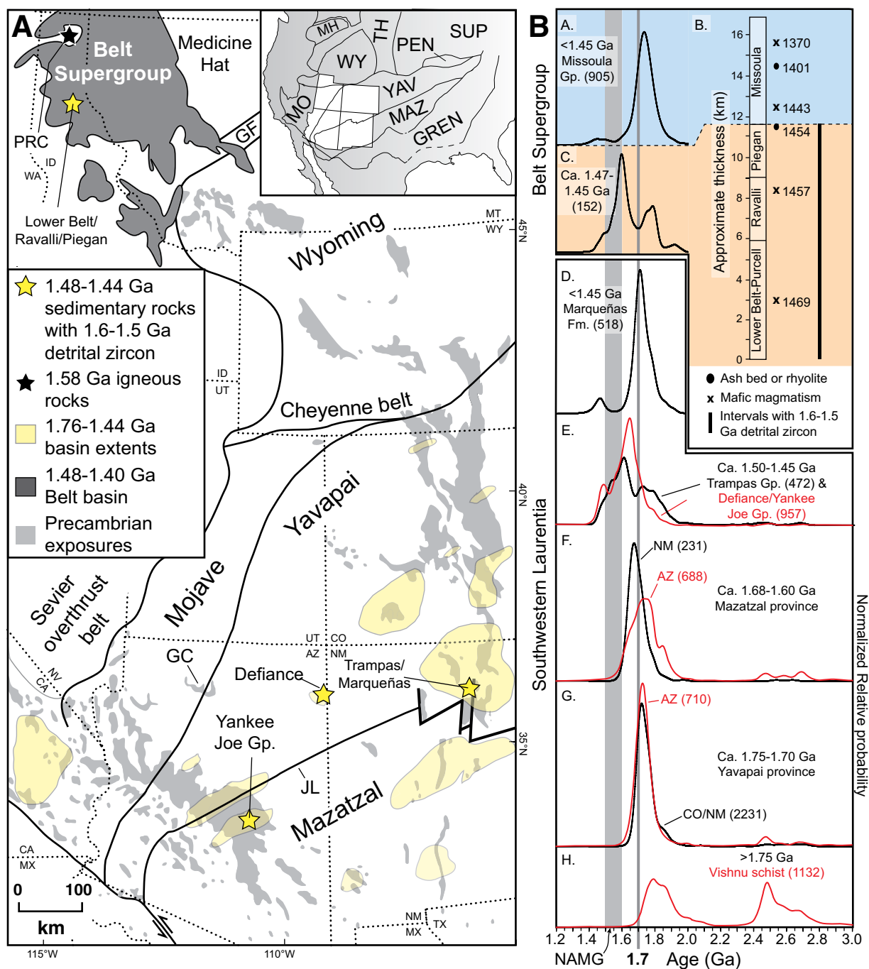
Figure 2. (A) Map showing Precambrian provinces (separated by solid lines) and rock exposures (light-gray shapes) in the western United States. Areas outlined in yellow show inferred extent of Paleoproterozoic and Mesoproterozoic sedimentary basins, and stars highlight localities discussed in the text. PRC—Priest River complex; GF—Great Falls tectonic zone; GC—Grand Canyon; JL—Jemez/Morenci Lineament; TG/MQ—Trampas Group and Marquēñas Formation. Inset shows: MH—Medicine Hat block; MO—Mojave; WY—Wyoming; TH—Trans-Hudson; PEN—Penokean; SUP—Superior; YAV—Yavapai; MAZ—Mazatzal; GREN—Grenville. (B) Compiled detrital zircon geochronologic data for the lower three units (orange, panel C) and upper unit (blue, panel A) of the Belt-Purcell Supergroup together with generalized stratigraphy and published depositional age constraints (panel B; Doughty and Chamberlain, 1996; Doughty et al., 1998; Sears et al., 1998; Evans et al., 2000; Ross and Villeneuve, 2003; Lewis et al., 2006; Link et al., 2007, 2013; Stewart et al., 2010). (C) Compiled detrital zircon geochronologic data and likely depositional age ranges from 1.75 to 1.45 Ga metasedimentary successions exposed in the southwestern United States; red probability density curve and labels indicate Arizona (AZ) localities, and black curves and labels indicate Colorado and/or New Mexico (CO/NM) localities (Jessup et al., 2005; Jones and Connelly, 2006; Amato et al., 2008; Jones et al., 2009, 2011; Shufeldt et al., 2010; Doe et al., 2012, 2013; Jones and Thrane, 2012; Daniel et al., 2013; Doe, 2014). Numbers in parentheses for detrital zircon age spectra indicate number of grains included in each age probability density curve. Note that the detrital zircon age spectra are all composites of multiple samples from previously published data sets referenced above, and the composite curves might mask statistically significant age populations from individual samples. NAMG—North American magmatic gap.
