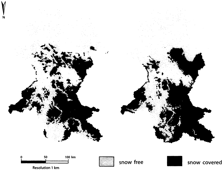
Fig. 1. Comparison between snow cover in the Weser catchment on February 14 th , 1994 as detected by NOAA-AVHRR (left) and modelled with ESCIMO (right). The percentage of snow covered raster elements in the NOAA-AVHRR image is 32%, whereas it is 36% in that computed by the model. The image-to-image comparison shows that the snow cover situation (snow covered or snow free, respectively) is correctly modelled for 84.2% of the raster elements (from Strasser 1998).
