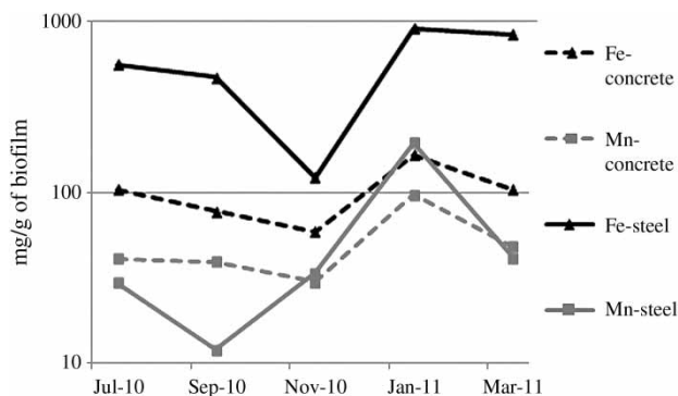
Figure 2 | Iron and manganese concentrations in DWTP biofilms.
