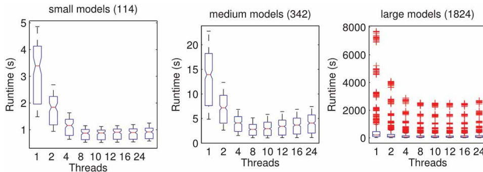
Figure 2 | Runtime of Achilles on TE testing 2,280 models of the set of synthetic generated water supply networks (CS1.1).
