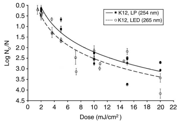
Figure 4 | Log reduction of E. coli K12 by irradiation from low-pressure lamps (254 nm) and LEDs (265 nm). Data lines represent logarithmic regression and error bars represent one standard deviation of the mean of quintuplicates.
