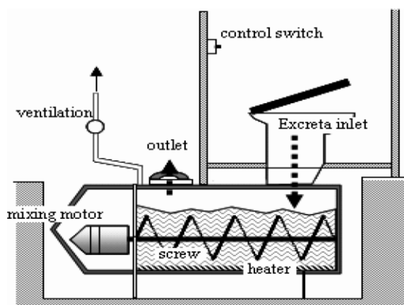
Figure 1 | The Bio-toilet.
