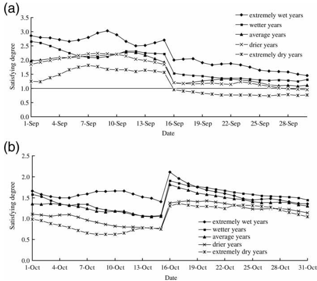
Figure 4 | Mean daily satisfying degree of the minimum ecological flow in five types of years (Scheme II): (a) September and (b) October.
