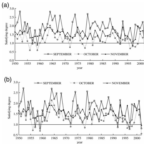
Figure 2 | Monthly satisfying degree of the minimum ecological flow for different years: (a) Scheme I and (b) Scheme II.
