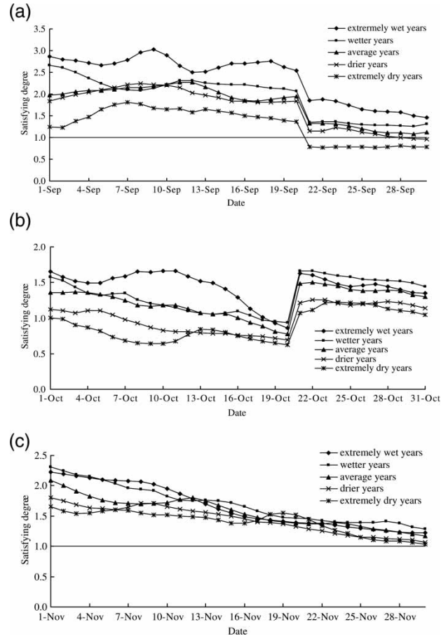
Figure 3 | Mean daily satisfying degree of the minimum ecological flow in five types of years (Scheme I): (a) September; (b) October and (c) November.
