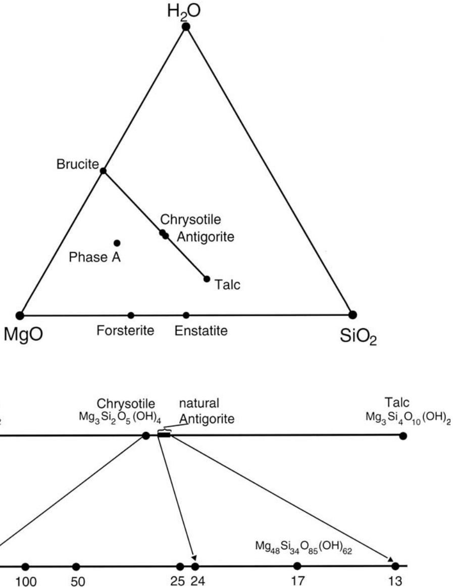
Fig. 1. Selected phases of the system MgO-SiO 2 -H 2 O (MSH) and enlarged projection of the tie-line brucite – talc with the range of chemical variations of natural antigorites according to Mellini et al. (1987), defined by m -values (see text).
