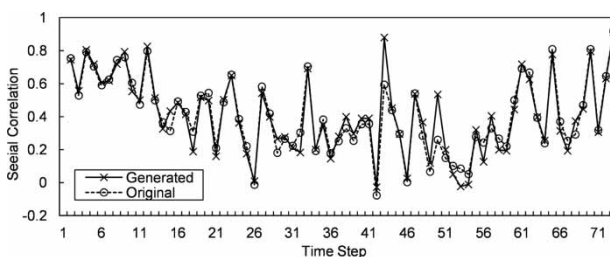
Figure 6 | Serial correlations of inflows generated by each five-daily time step.
