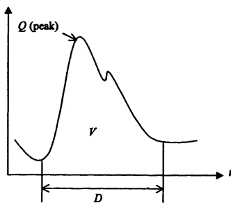
Fig. 1. Characteristic values of a flood event.
