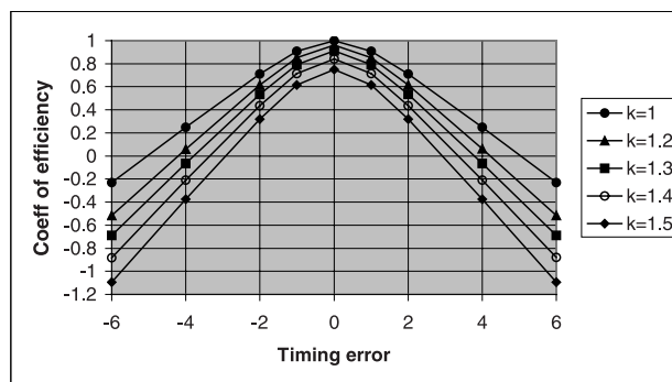
Figure 6 | The effect of volumetric and timing errors on the coefficient of efficiency based upon the first differences of the computed and observed flows; volumetric errors range from 0–50% overestimation of the observed runoff volume.
