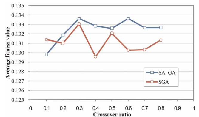
Figure 8 | Average fitness values corresponding to optimal parameters of SAC-SMA model calibrated by SA_GA and SGA with various crossover ratios.
