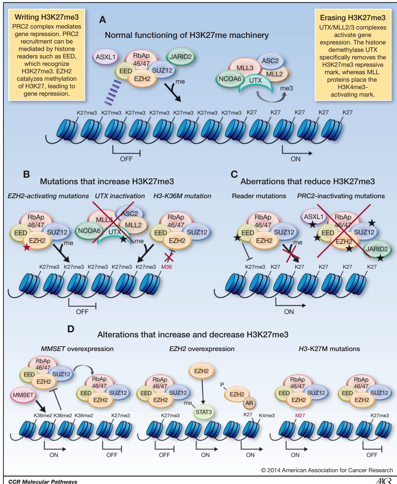
Figure 1. A, H3K27me3 writing is carried out by the PRC2 complex accompanied by accessory proteins such as JARID2 and ASXL1. One mechanism of PRC2 recruitment is the recognition of H3K27me3 by the PRC2-component EED, which leads to self-propagation of this mark. EZH2 catalyzes H3K27 methylation, leading to H3K27me3 and gene repression. H3K27me3 erasing is done by the histone demethylase UTX, which specifically removes the repressive mark H3K27me3, leading to gene activation. H3K27me3 erasing is done by the histone demethylase UTX, which specifically removes the repressive mark H3K27me3, leading to gene activation. B, alterations that produce increases in the levels of H3K27me3 include activating mutations of EZH2, inactivating mutations of the histone demethylase UTX that lead to failure in the removal of this mark, and K36M mutations in histone H3. (Continued on the following page.)
