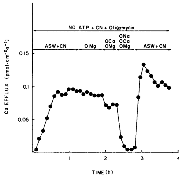
FIGURE 9. The effect of external magnesium, calcium, and sodium on the calcium efflux in the absence of internal ATP. Abscissa: time in hours. Ordinate: calcium efflux in \text{pmol}\cdot\text{cm}^{-2}\cdot\text{s}^{-1} . [\text{Ca}]_i = 0.3 \mu\text{M} . T^\circ = 22^\circ\text{C} . Axon diameter: 400 \mu\text{m} .
