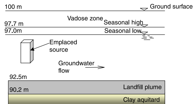
Figure 1 | Sketch of tracer test at Borden Site, Ontario, Canada.
