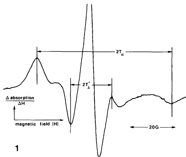
FIGURE 1 First derivative ESR spectrum at 25°C of 5DS-labeled erythrocytes from a CHS patient. The hyperfine splitting parameters 2T_{\parallel} and 2T_{\perp} are the separation between outer and inner extrema, respectively, and are used in the calculation of order parameter.
