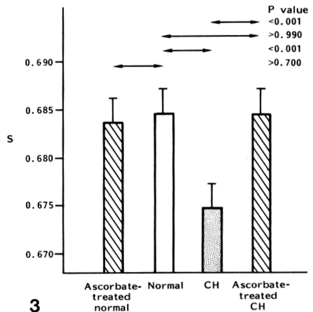
FIGURE 3 Order parameter at 25°C for 5DS-labeled erythrocytes from three normal humans and the CHS patient. Incubation and labeling conditions are described in Materials and Methods. Final concentration of ascorbate was 0.01 M. Bars indicate 2 SE above the mean. Values are from analysis of nine or more samples from three separate experiments. P values are for the probability that a null hypothesis comparing the indicated values is true.
