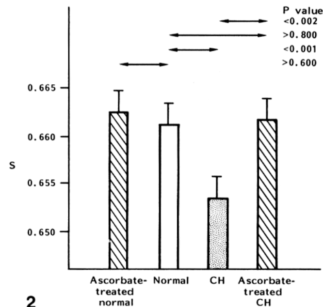
FIGURE 2 Order parameters at 23°C for 5DS-labeled erythrocytes from normal and CHS mice. Incubation and labeling conditions are described in Materials and Methods. Final concentration of ascorbate was 0.01 M. Bars indicate 2 SE above the mean. Values are from analysis of 12 or more samples from three separate experiments. P values are for the probability that a null hypothesis comparing the indicated values is true.
