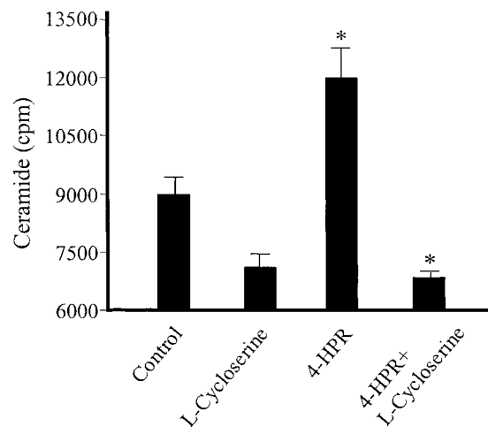
Fig. 3. Effect of SPT inhibitor L-cycloserine on 4-HPR-induced ceramide generation. CHLA-90 cells cultured in 6-well plates were treated with L-cycloserine (5 mM), 4-HPR (10 \mu\text{M} ), or both agents in medium containing [ ^3\text{H} ]palmitic acid for 4 h. Radiolabeled ceramide was resolved from the total cell lipids by TLC and quantitated by LSC. *, P < 0.01 . The Y axis represents cpm of ceramide per 500,000 cpm of total lipid tritium.
