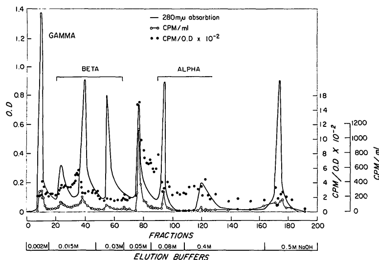
Fig. 1. The calf lens protein was fractionated on a 15 Cm. DEAE column by stepwise elution. All buffers were prepared by the dilution of 0.500M ( \text{NaH}_2\text{PO}_4, \text{K}_2\text{HPO}_4 ), pH 6.85 \pm 0.05 . Fractions were collected in 15 ml. aliquots, and 0.5 ml. aliquots were used for counting.
