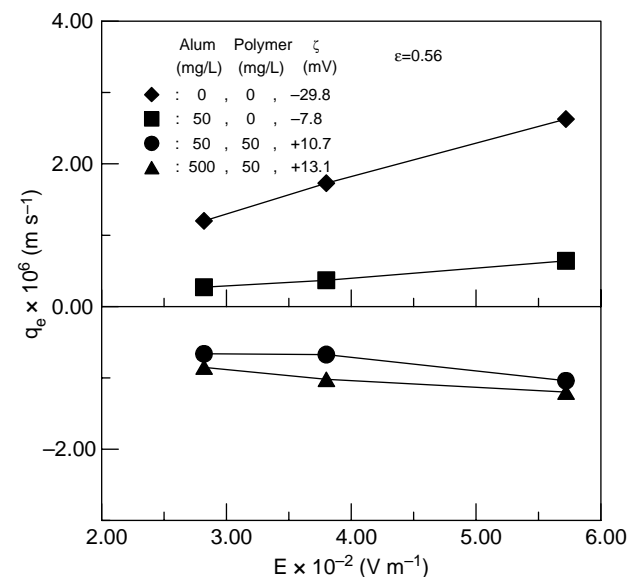
Figure 6 | Electroosmotic flux through bed packed with cationic flocculant conditioned alum-coagulated slurry.
