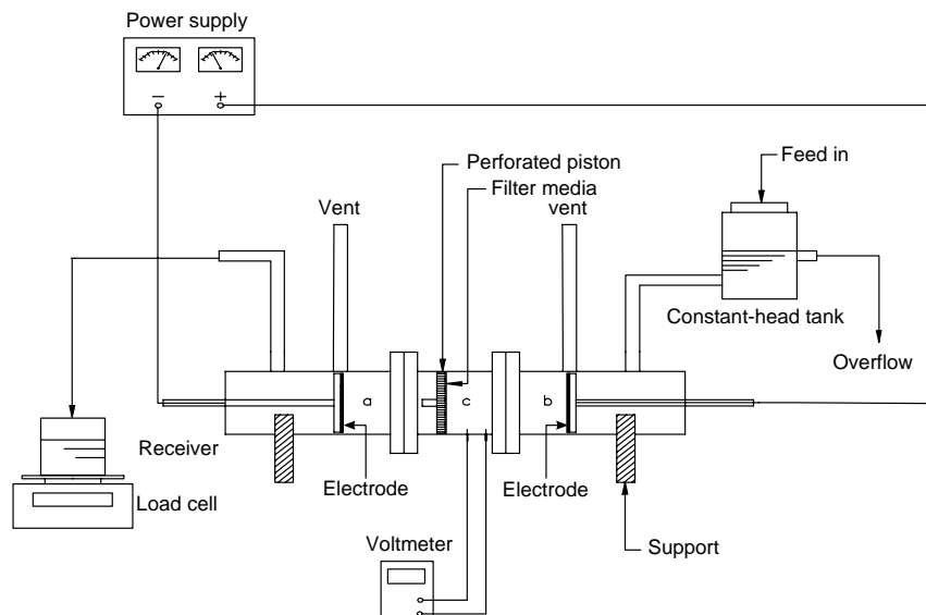
Figure 1 | Experimental set-up to measure the electroosmotic flow through the sludge bed.
