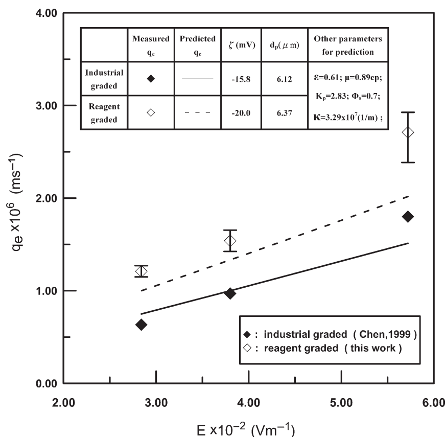
Figure 2 | Comparison between measured values and model predictions for the electroosmotic flux of kaolin beds at 10^{-4} M KCl. (Error bars depict the maximum and minimum flux from duplicated tests at each electric field strength.)
