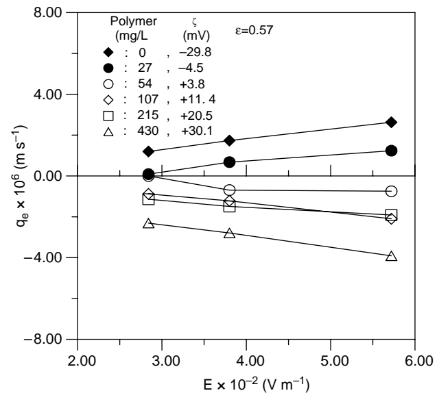
Figure 5 | Electroosmotic flux through bed packed with polymer flocculated slurry.
