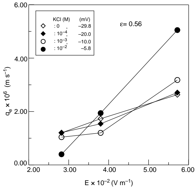
Figure 3 | Effect of KCl concentration on the electroosmotic flux of a kaolin bed.
