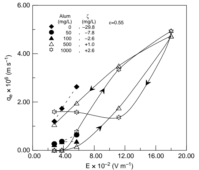
Figure 4 | Electroosmotic flux through bed packed with alum-coagulated slurry.
