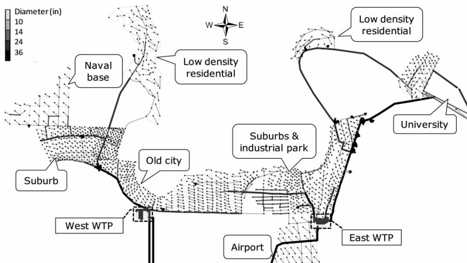
Figure 3 | Mesopolis WDS. Different land uses have distinct water demand patterns in the hydraulic model.
