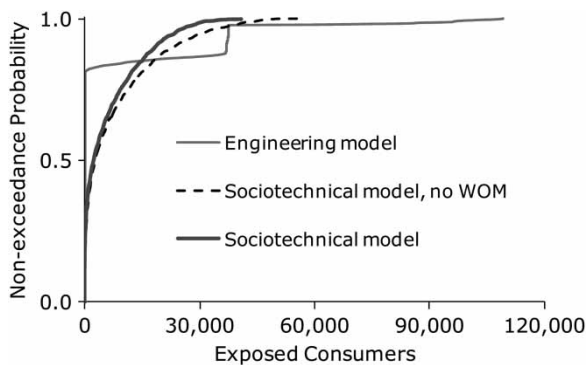
Figure 4 | MCS results for engineering and sociotechnical models. WOM indicates word-of-mouth mechanism.
