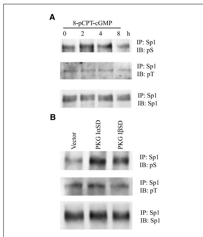
Figure 6. PKG phosphorylates Sp1 at serine site(s). A , SW480 cells were treated with 250 \mu\text{mol/L} 8-pCPT-cGMP for the indicated times and cell lysates were used for immunoprecipitation assays with an anti-Sp1 antibody. Phospho-serine (pS) bands were visualized by using an anti-phospho-serine antibody. The same membrane was stripped and reprobed with an anti-phospho-threonine (pT) antibody and an anti-Sp1 antibody, consecutively. B , SW480 cells were transfected with the empty vector, PKG I \alpha SD, and PKG I \beta SD plasmids, as indicated. Thirty hours after transfection, cell lysates were used for immunoprecipitation assays and subsequent Western blot analysis, as described in A . All experiments were repeated three times and representative results are shown.
