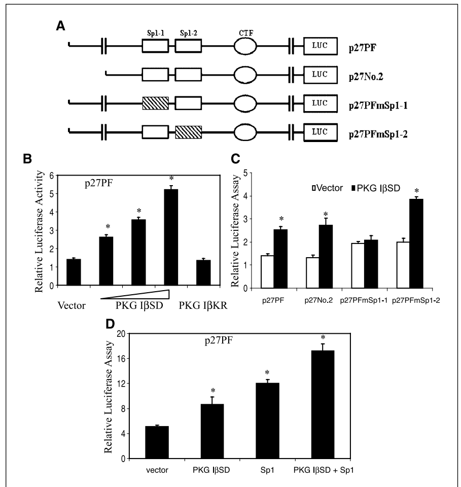
Figure 4. PKG increased p27 promoter luciferase reporter activity. A, schematic diagrams of p27 promoter luciferase reporter (p27PF) and its mutants. B, luciferase assays were conducted as described in Fig. 3B except that p27PF was used as the reporter instead of pWWP. P < 0.05, versus control. C, luciferase assays were conducted as described in Fig. 3C except that p27PF, p27No.2, p27PFmSp1-1, and p27PFmSp1-2 were used to replace pWWP, pWWP124, and pWWP101. P < 0.05, versus control. D, the p27PF reporter was cotransfected with the empty vector, PKG I \beta SD plasmid, and Sp1 plasmid, as indicated. Luciferase assays were done as described in Fig. 3D. P < 0.05, versus control.
