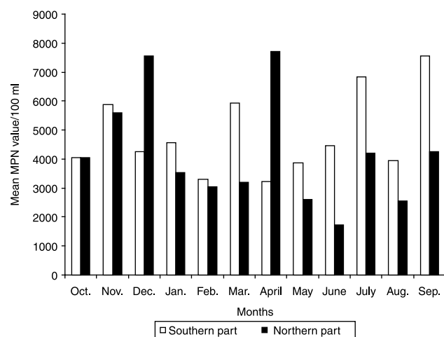
Figure 2 | Prevalence of faecal indicator bacteria in northern and southern part of the salt water regulator in Vembanadu Lake during 2004 to September 2005.
