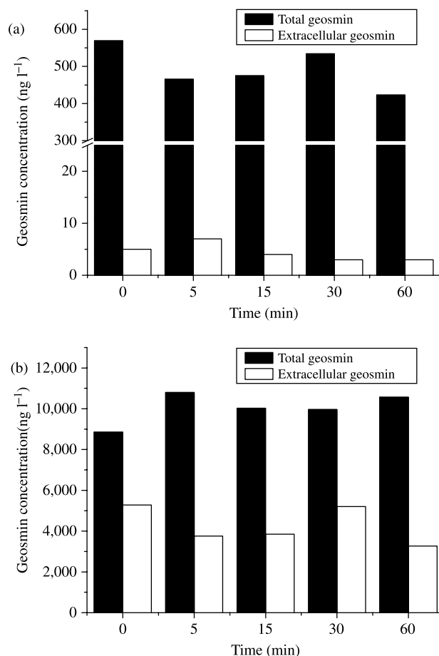
Figure 3 | Total and extracellular geosmin concentrations after treatment with potassium permanganate (0.5 mg l -1 ) using Anabaena circinalis at numbers of: (a) 2,000 cells ml -1 ; and (b) 50,000 cells ml -1 .
