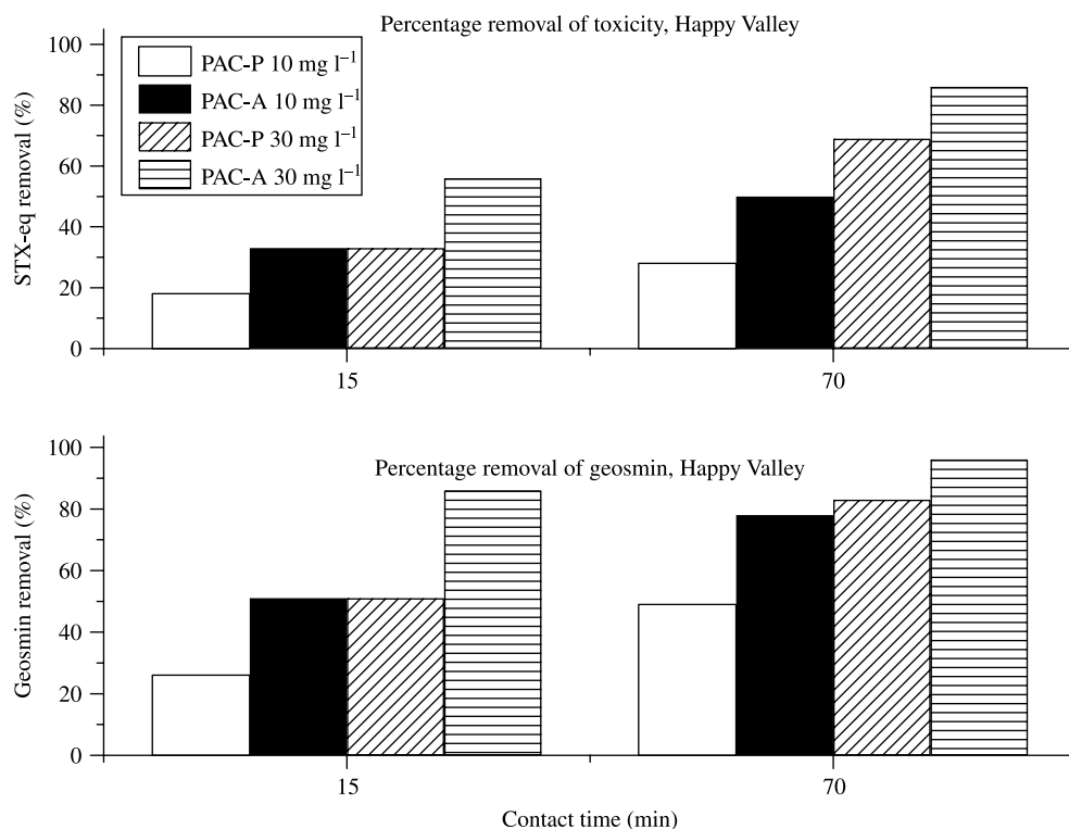
Figure 8 | Percentage removals of geosmin and saxitoxin toxicity equivalent (STX-eq) in Happy Valley water using two PACs at doses of 10 and 30 \text{ mg l}^{-1} .
