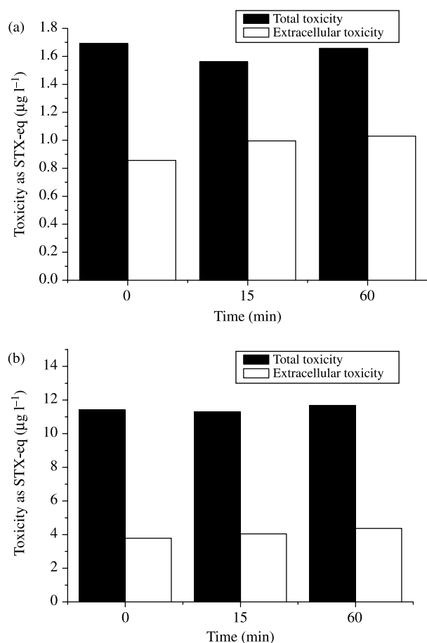
Figure 4 | Total and extracellular saxitoxins concentrations, expressed as STX-eq, after treatment with potassium permanganate ( 0.5 \text{ mg l}^{-1} ) using Anabaena circinalis at numbers of: (a) 2,000 cells \text{ml}^{-1} ; and (b) 50,000 cells \text{ml}^{-1} .
