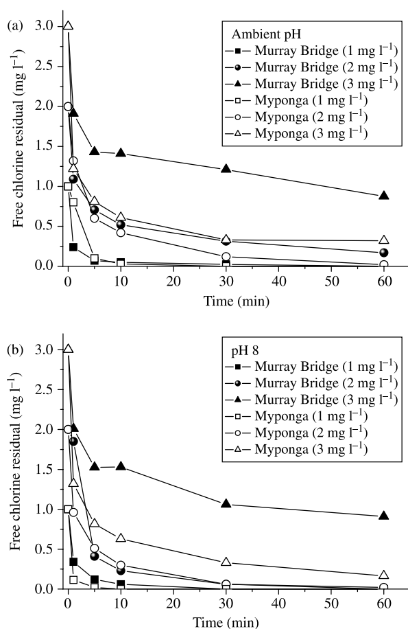
Figure 9 | Chlorine decay as a function of time in Murray Bridge and Myponga treated waters at: (a) ambient pH; and (b) pH 8.
