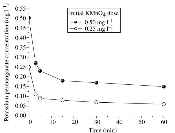
Figure 2 | Decay of potassium permanganate in Myponga Reservoir water using doses of 0.25 and 0.50 mg l -1 .
