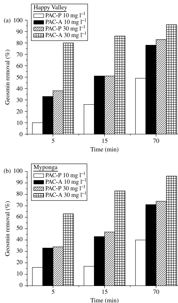
Figure 5 | Comparison of geosmin removal using two PACs at doses of 10 and 30 \text{ mg l}^{-1} in: (a) Happy Valley Reservoir water; and (b) Myponga Reservoir water.
