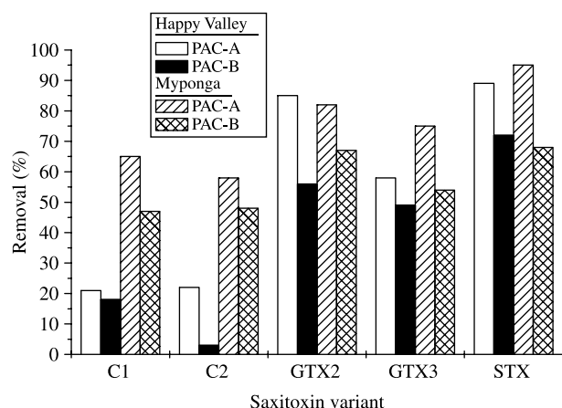
Figure 7 | Percentage removal of the individual saxitoxin variants by the two PACs in Happy Valley and Myponga waters (PAC dose of 30 \text{ mg l}^{-1} , contact time of 70 min).
