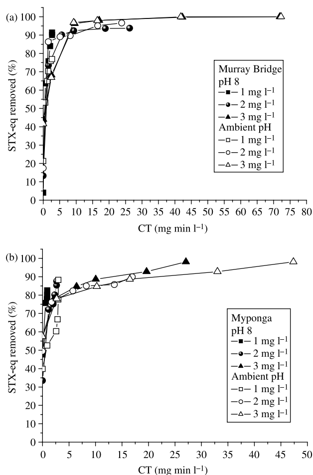
Figure 10 | Saxitoxin oxidation, expressed as STX-eq, as a function of CT using chlorine doses of 1, 2 and 3 mg l -1 in: (a) Murray Bridge treated water; and (b) Myponga treated water.
