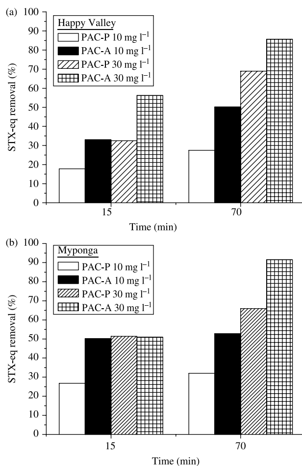
Figure 6 | Comparison of saxitoxin toxicity equivalent (STX-eq) removal using two PACs at doses of 10 and 30 mg l -1 in: (a) Happy Valley Reservoir water; and (b) Myponga Reservoir water.
