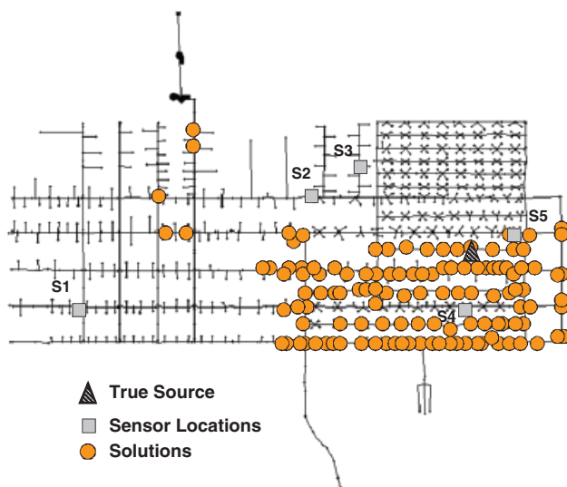
Figure 9 | Locations of candidate nodes at 12:30 p.m. (based on 10-min observations).
